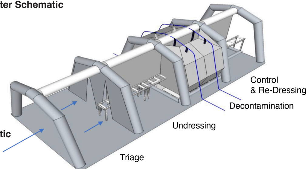
Losberger Decon TAG 30 Shelter Schematic
